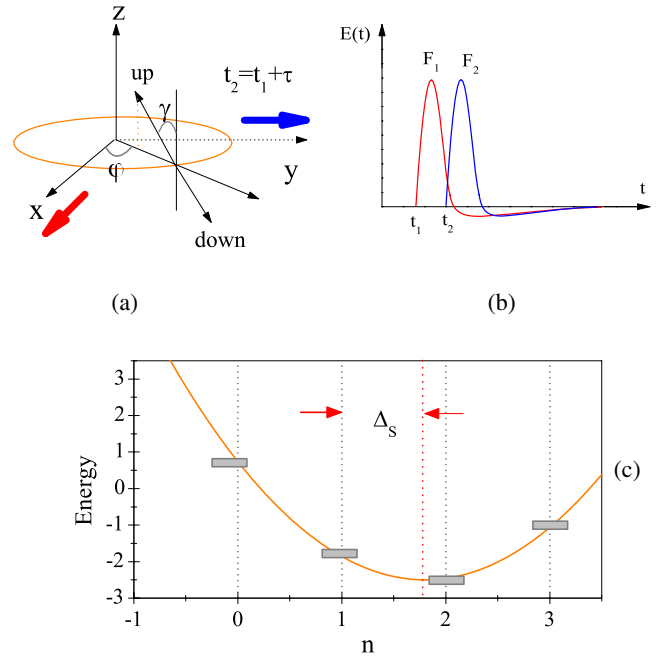
Figure 1. (a) A schematic graph of the geometry, spin configuration and the applied pulses is shown. (b) Time-delayed asymmetric pulses are schematically drawn. (c) Energy spectrum for a ring with spin-orbit interaction. \Delta_S defines the distance between the spectrum symmetry axis and the smallest nearest integer.
