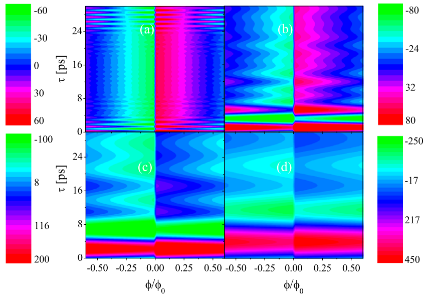
Figure 3. Contour plots of TCC on \phi and \tau are shown for different radii of the ring. a = 100 nm, 200 nm, 300 nm and 400 nm in (a), (b), (c) and (d), respectively. The other parameters are N = 100, \gamma = 0^\circ, F_1 = F_2 = 500 V cm ^{-1} .
