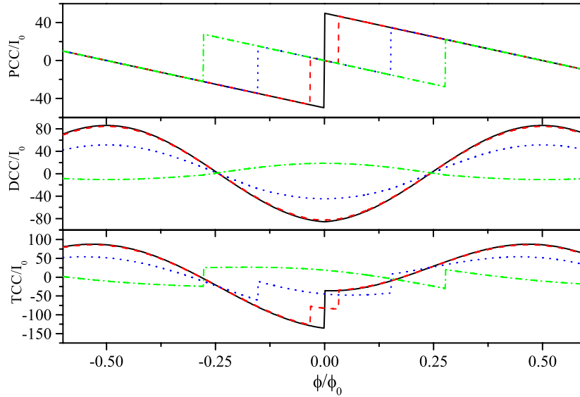
Figure 2. Persistent charge current (PCC), dynamic charge current (DCC) and total charge current (TCC) are shown in (a), (b) and (c), respectively. The spin orbit angles are \gamma = 0^\circ, -20^\circ, -40^\circ and -50^\circ for the solid lines, the dashed lines, the dotted lines and the dashed-dotted lines respectively in all graphs. The other parameters are N = 100, a = 100 nm, \tau = 26.3 ps, F_1 = F_2 = 1 kV cm ^{-1} .
