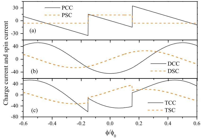
Figure 4. PCC and PSC, DCC and DSC, and TCC and TSC are shown in (a), (b) and (c), respectively. The solid lines are the charge current, and the dashed lines are the spin current. \gamma = -40^\circ , the other parameters are the same as in figure 2.
