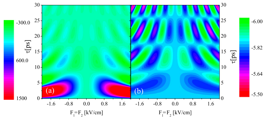
Figure 5. TCC (a) and TSC (b) versus pulse strengths F_1 = F_2 and delay time \tau . \gamma = -40^\circ , \phi = 0.2 . Other parameters are N = 100 , a = 400 nm.
